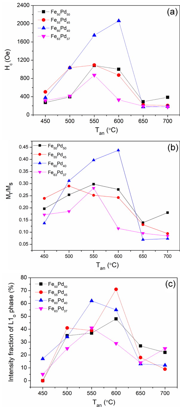
Fig. 8 a Coercivity ( H_C ), b squareness ratio ( M_r/M_s ), and c intensity fraction of L1_0 phase versus annealing temperature for \text{Fe}_x\text{Pd}_{100-x} ( x = 50, 55, 60 and 63 ) nanoparticles measured at room temperature.
